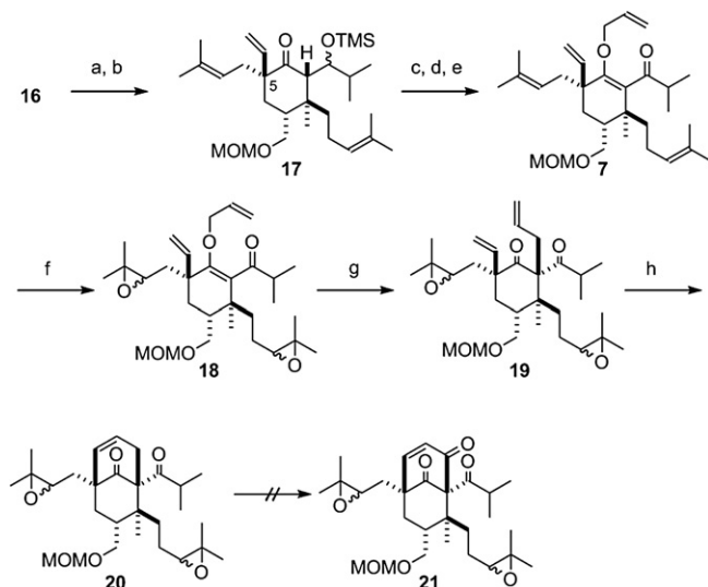
Scheme 3. Claisen rearrangement–RCM approach toward bicyclic core. Reagents and conditions: (a) LDA, TMEDA, acetaldehyde, THF, >99%. (b) Martin sulfuran, toluene/CH 2 Cl 2 . (c) HF·Py, pyridine, THF, 73% (two steps). (d) DMP, CH 2 Cl 2 , 90%. (e) KHMDS, HMPA, allyl iodide, THF, 89%. (f) m -CPBA, CH 2 Cl 2 , 74%. (g) toluene, 180 °C, 46%. (h) Hoveyda–Grubbs second cat., toluene, 74%.
