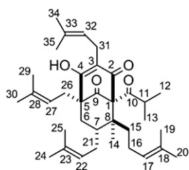
Figure 3. Numbering of hyperforin.
