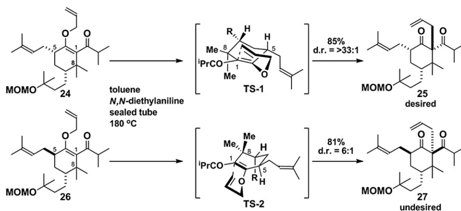
Scheme 5. Selectivity of Claisen rearrangement.
