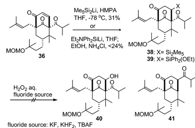
Scheme 7. Tamao–Fleming oxidation approach.
