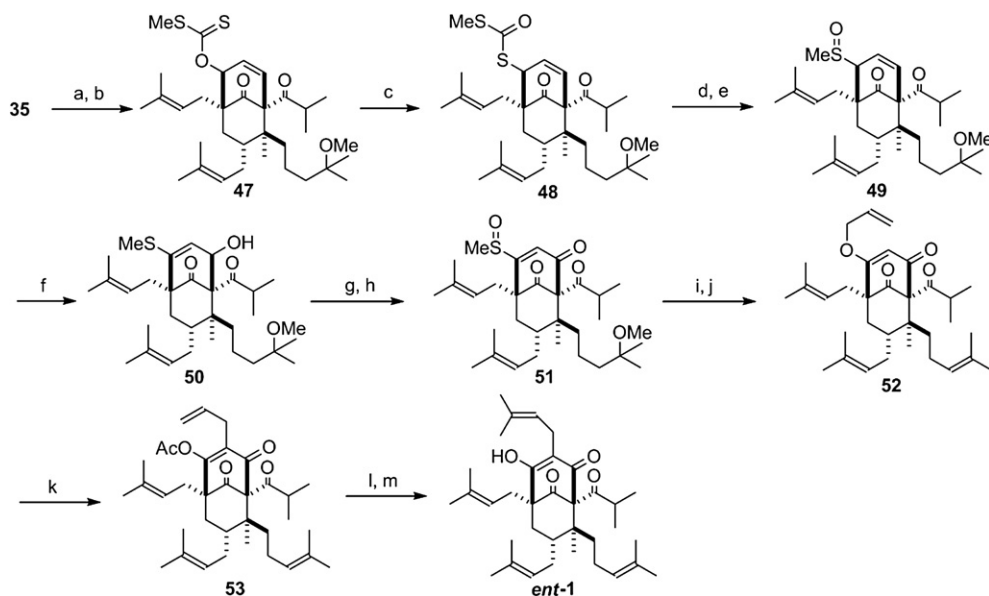
Scheme 9. Completion of the total synthesis. Reagents and conditions: (a) \text{NaBH}_4 , MeOH, 95% (dr >33:1). (b) \text{CS}_2 , NaH, THF; MeI, >99%. (c) toluene, 150^\circ\text{C} . (d) EtSLi, THF; MeI, \text{NEt}_3 , 98% (two steps). (e) \text{NaBO}_3 \cdot 4\text{H}_2\text{O} , AcOH (dr=1.3:1), 95%. (f) TFAA, 2,6-di- tert -butylpyridine, \text{CH}_2\text{Cl}_2 , -40^\circ\text{C} ; \text{H}_2\text{O} , 65% (dr >33:1). (g) \text{H}_2\text{O}_2 , HFIP, 87% (dr=9:1). (h) DMP, \text{CH}_2\text{Cl}_2 , 86%. (i) Amberlyst 15DRY, toluene, 55%. (j) LiH, allyl alcohol, 67%. (k) \text{Pd}_2\text{dba}_3 \cdot \text{CHCl}_3 (10 mol %), (S)- tol -BINAP (20 mol %), THF; \text{Ac}_2\text{O} , pyridine, 50%. (l) Hoveyda–Grubbs second cat. (15 mol %), 2-methyl-2-butene, \text{CH}_2\text{Cl}_2 , 34%. (m) \text{K}_2\text{CO}_3 , MeOH, 94%.
