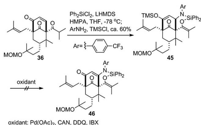
Scheme 8. Intramolecular addition of silyl aniline.
