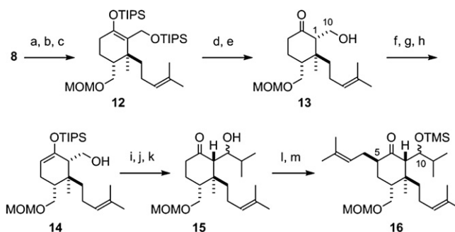
Scheme 2. Conversion of catalytic asymmetric Diels–Alder product. Reagents and conditions: (a) EtSLi, THF, 96%. (b) LAH, THF, 99%. (c) MOMCl, TBAI, i -Pr 2 NEt, CH 2 Cl 2 , 94%. (d) TBAF, AcOH, THF. (e) HF·Py, pyridine, THF, 91% (two steps; dr =1:1). (f) TMSCl, NEt 3 , CH 2 Cl 2 . (g) TIPSOTf, i -Pr 2 NEt, CH 2 Cl 2 . (h) K 2 CO 3 , MeOH. (i) TPAP (10 mol %), NMO, MS 4 Å, CH 3 CN/CH 2 Cl 2 . (j) 2-bromopropane, Li, THF ( dr =5:1). (k) TBAF, AcOH, THF, 58% (six steps). (l) TMSCl, imidazole, DMF, 94%. (m) LDA, HMPA, prenyl bromide, THF, 89%.
