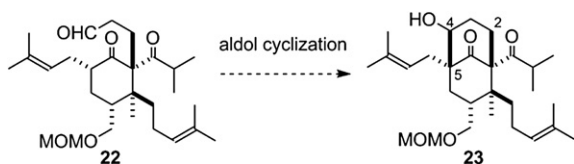
Scheme 4. Aldol cyclization approach.
