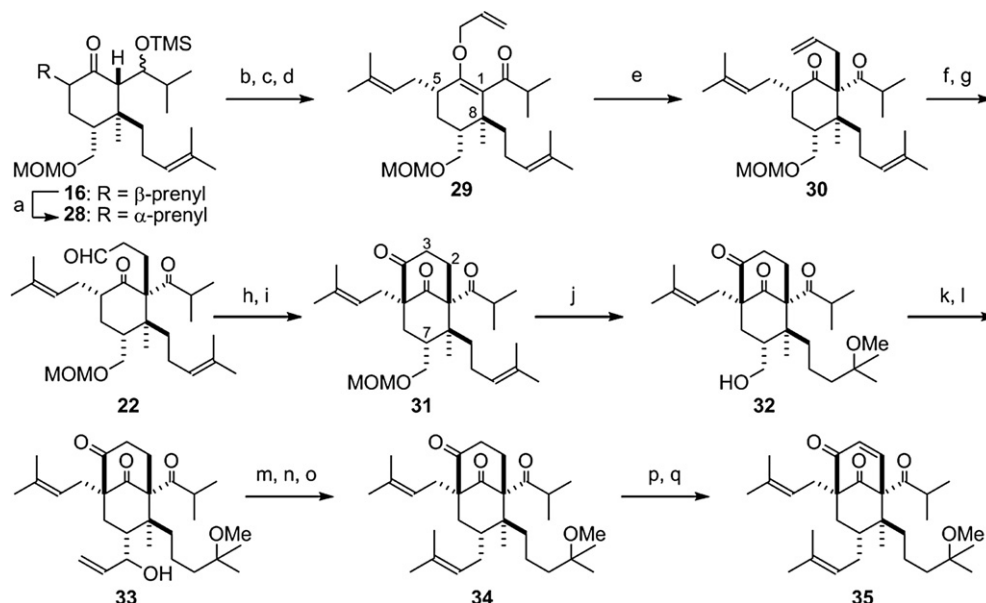
Scheme 6. Construction of the bicyclic core. Reagents and conditions: (a) LDA, THF; \text{NH}_4\text{Cl} aq, 88% (dr >33:1). (b) HF·Py, pyridine, THF. (c) DMP, \text{CH}_2\text{Cl}_2 , 96% (two steps). (d) NaHMDS, allyl bromide, HMPA, THF, >99%. (e) toluene, N,N -diethylaniline, 170 °C, >99% (dr=12:1). (f) (\text{Sia})_2\text{BH} , THF; \text{H}_2\text{O}_2 aq, NaOH aq, EtOH, 81%. (g) DMP, \text{CH}_2\text{Cl}_2 , 91%. (h) NaOEt, EtOH. (i) DMP, \text{CH}_2\text{Cl}_2 , 86% (two steps). (j) (+)-CSA, MeOH, 66% (three cycles). (k) (\text{COCl})_2 , DMSO, \text{CH}_2\text{Cl}_2 ; \text{NEt}_3 , 95%. (l) vinylmagnesium bromide, THF, 92% (dr >33:1). (m) \text{Ac}_2\text{O} , DMAP, i -Pr 2 NEt, \text{CH}_2\text{Cl}_2 , 98%. (n) \text{Pd}(\text{PPh}_3)_4 (20 mol %), \text{HCO}_2\text{NH}_4 , toluene, 95%. (o) Hoveyda–Grubbs second cat. (15 mol %), 2-methyl-2-butene, \text{CH}_2\text{Cl}_2 , >99%. (p) TMSCl, \text{NEt}_3 , DMAP, \text{CH}_2\text{Cl}_2 , 84%. (q) \text{Pd}(\text{OAc})_2 , DMSO, \text{O}_2 , >99%.
