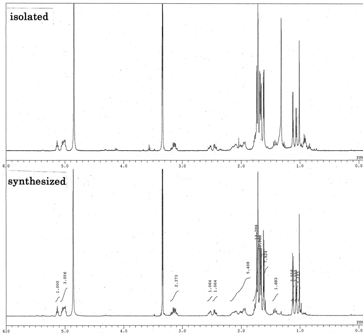
Figure 2. ^1\text{H} NMR of hyperforin.
